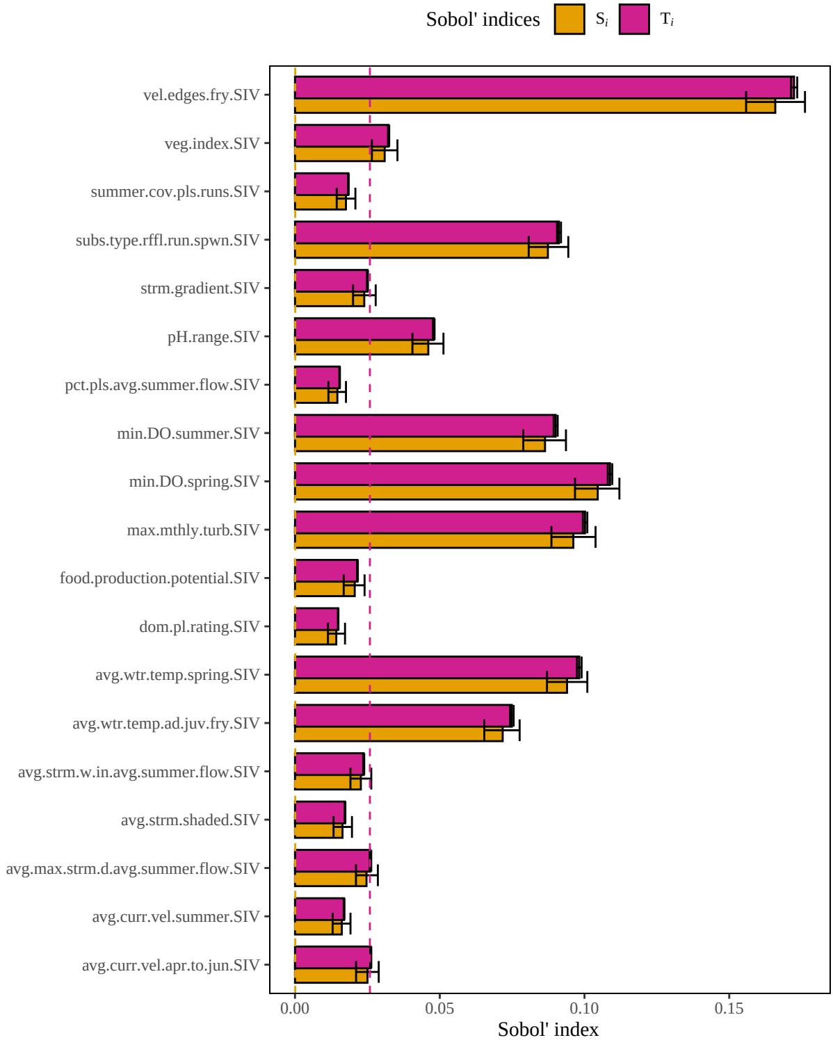
Figure 5. Results of a sensitivity analysis for the creekchubRivLargerStrmDistMt5km model based on a geometric mean structure. Dashed lines represent baseline numerical approximation error for S_i and T_i ( i.e. , dummy variables).
