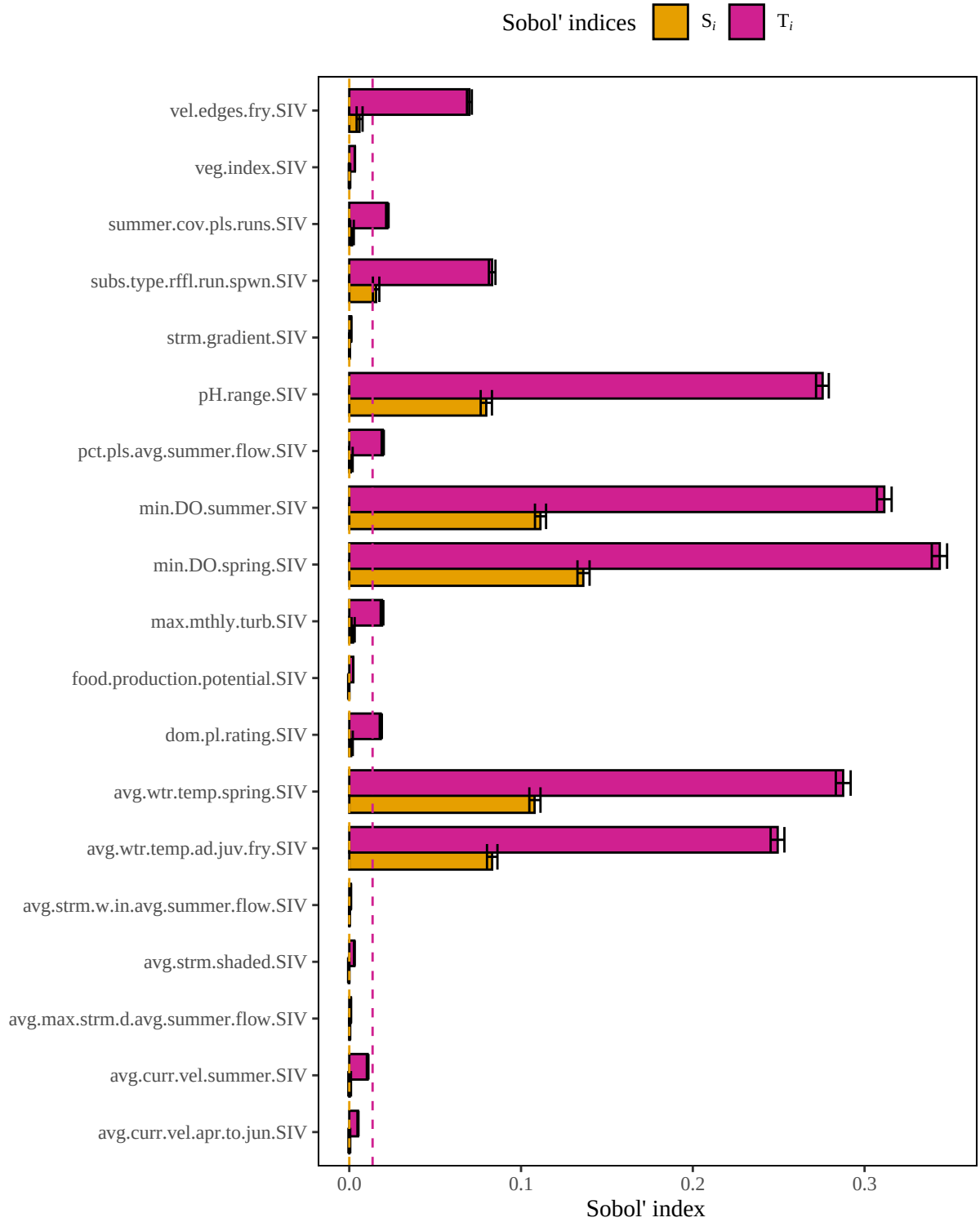
Figure 3. Results of a sensitivity analysis for the creekchubRivLargerStrmDistMt5km model based on the original author-specified model outlined in McMahon (1982). Dashed lines represent baseline numerical approximation error for S_i and T_i ( i.e. , dummy variables).
