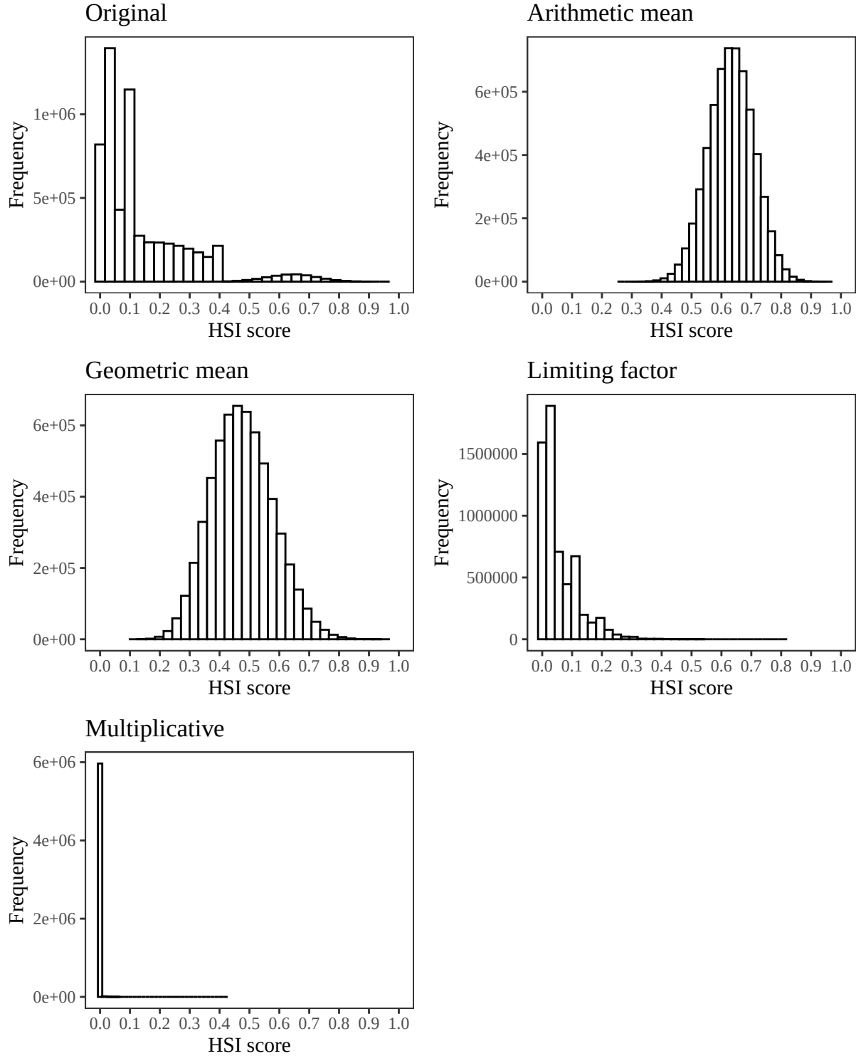
Figure 2. Empirical distributions of HSI scores for the creekhubRivLargerStrmDistMt5km model using the original author-specified model equation from McMahon (1982), and an arithmetic mean, geometric mean, limiting factor, and multiplicative structure incorporating all SIV variables. Note differences in the y axis.
