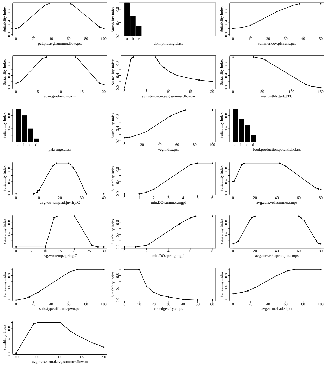
Figure 1. Suitability index graphs for variables included in the creekchubRivLargerStrmDistMt5km model in ecorest.
